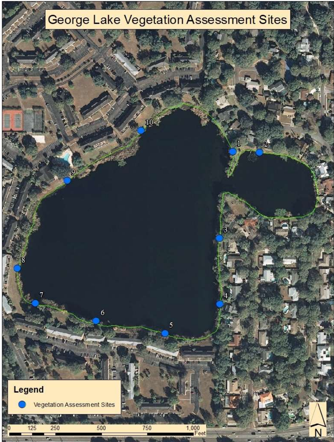
Figure 3. Vegetation assessment site map for George Lake
