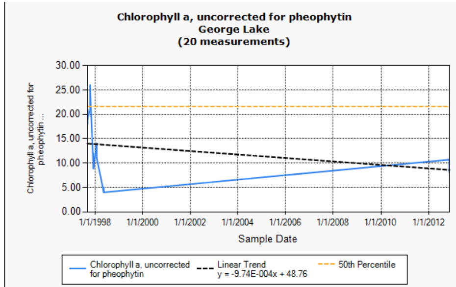
Figure 8. Period of Record Chlorophyll a graph for George Lake viii . ix
