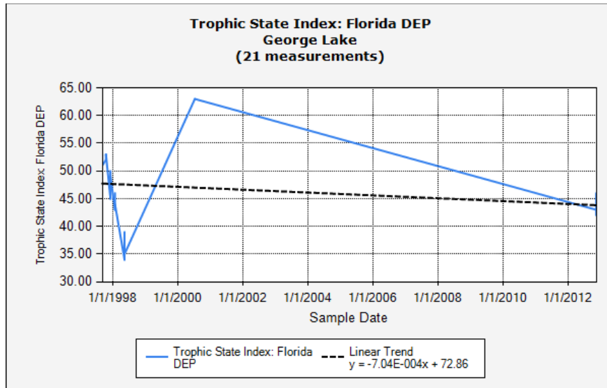
Figure 7. Period of Record Trophic State Index (TSI) graph for George Lake vi vii
